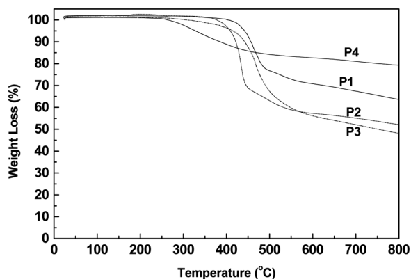
FIGURE 1 TGA curves of alternating copolymers.
