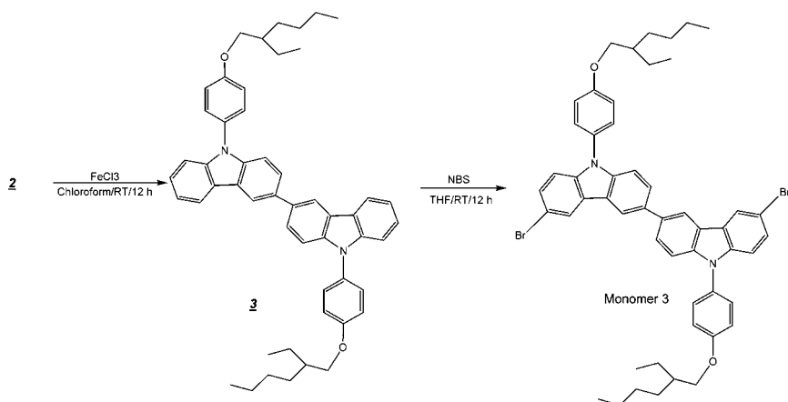
SCHEME 3 Synthetic route to monomer 3.
