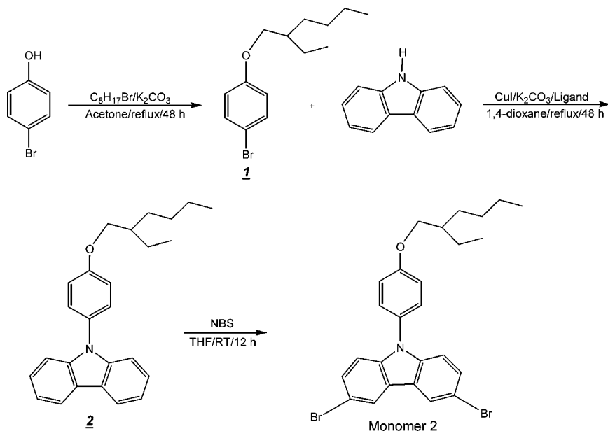
SCHEME 2 Synthetic route to monomer 2.
