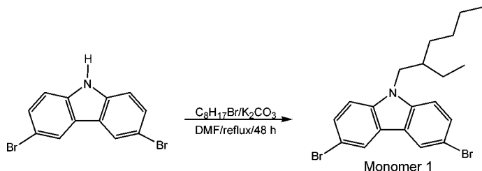
SCHEME 1 Synthetic route to monomer 1.
