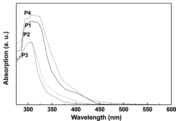
FIGURE 2 UV-Vis absorption spectra of alternating copolymers.
