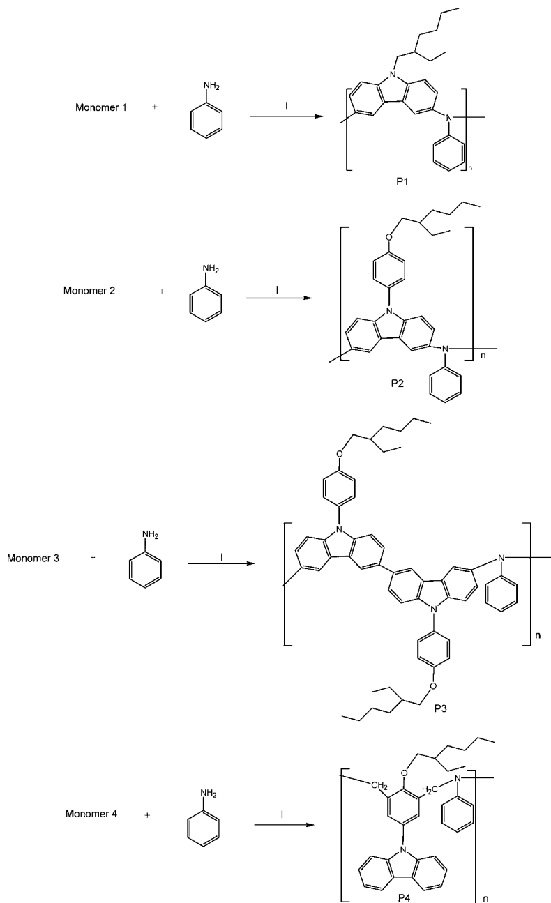
SCHEME 5 Polymerizations via palladium catalyzed polycondensation; Reaction condition (I): Toluene, NaO- t -Bu, Pd 2 (dba) 3 , P( t -Bu) 3 , 100°C.
