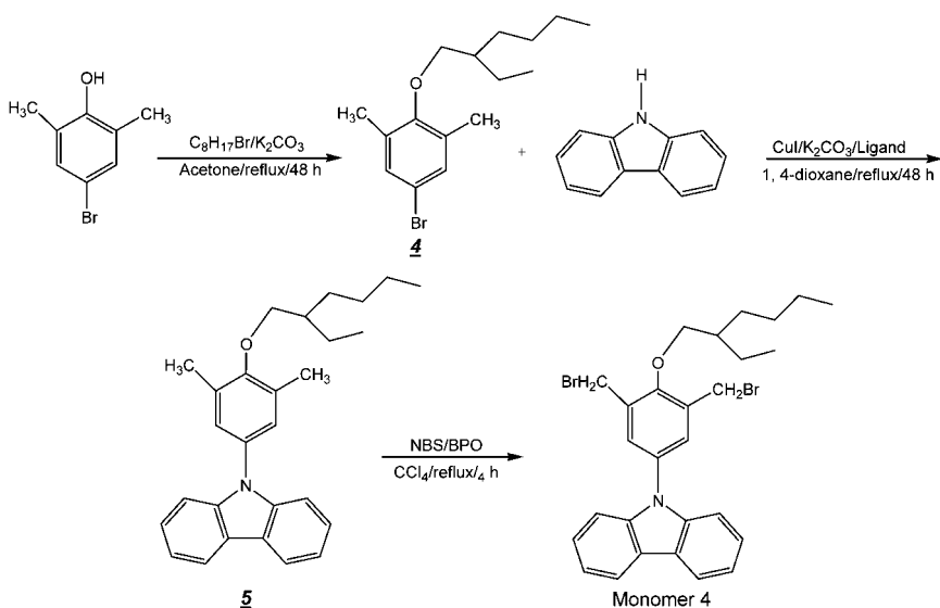
SCHEME 4 Synthetic route to monomer 4.
